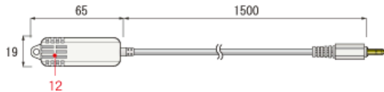
HHA-3151 (Temperature/Humidity Sensor High-Precision Type)
